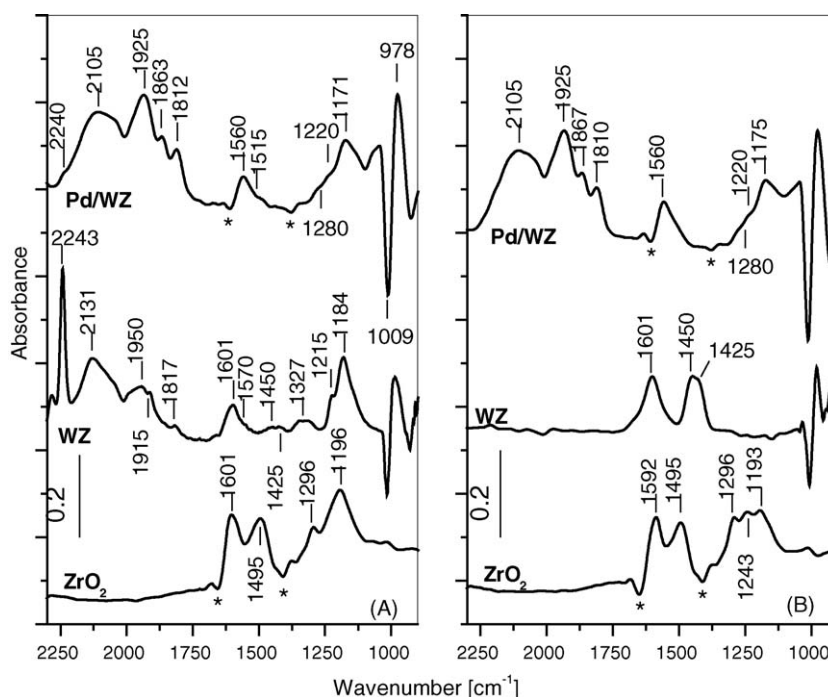
Fig. 4. (A) FT-IR spectra of NO (1.33 kPa) adsorbed for 30 min at room temperature on the samples studied. The gas phase spectra are subtracted. (B) After evacuation for 15 min at room temperature. The negative bands marked by asterisks are due to residual carbonates, which are removed by the \text{NO}_x species.
